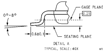
8-Pin Molded TSSOP, JEDEC (MT8) NS Package Number MTC08
