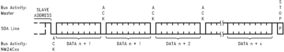
FIGURE 10. Sequential Read
