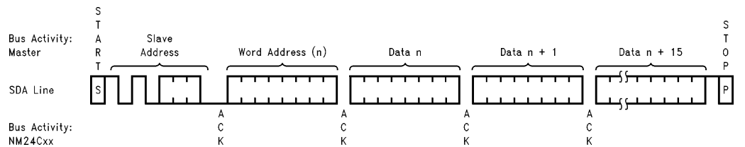
FIGURE 7. Page Write
